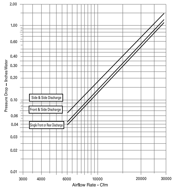
Chart PD-13. Airside Pressure Drop, Low Height Discharge Plenum 42 to 80 Ton Unit
